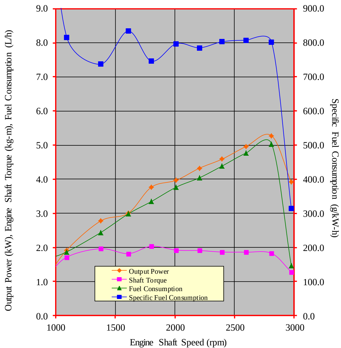
Figure 3. Performance characteristic curves of the FUCHAI R180N diesel engine
