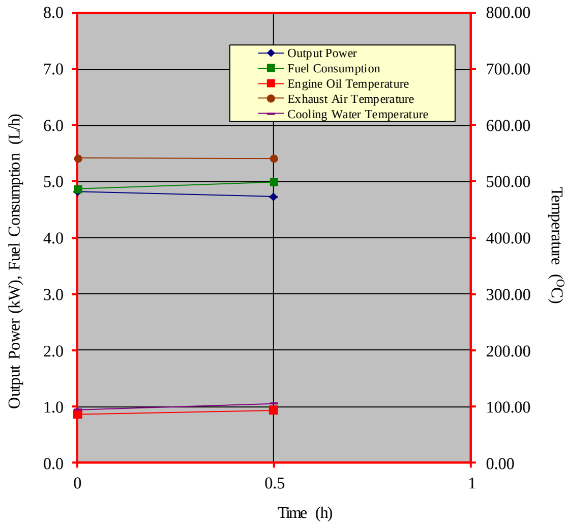
Figure 4. Performance characteristic curves during the continuous running test of the FUCHAI R180N diesel engine
